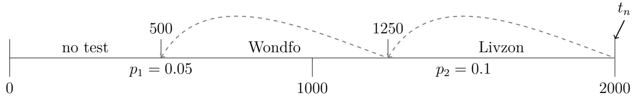
Figure 3: Optimal allocation and optimal replacement chain caused by replacement of one Livzon test with the “sensitive” test t_n .
